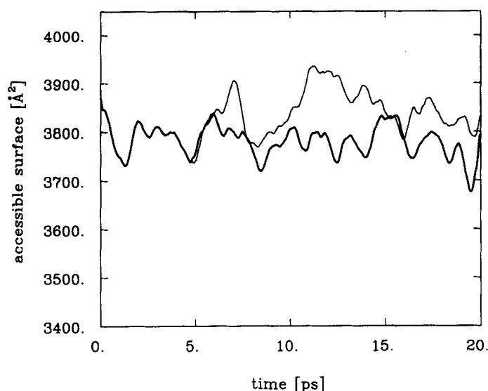
Figure 7 Time development of total solvent accessible surface of BPTI for molecular dynamics simulations A and B. The definition of solvent accessible surface is given in Section 2.1. The thick line refers to simulation A (protein in vacuum, full range electrostatic interactions are taken into account, parameters see Section 3.1), the thin line refers to simulation B (protein in solution, parameters for simulation and discretisation see Section 3.2 and 2.2.4). Both simulations started with the same protein structure (see definition of simulations A and B in Section 3.1 and 3.2). In simulation B, screening was switched on instantaneously at t = 5 ps.
