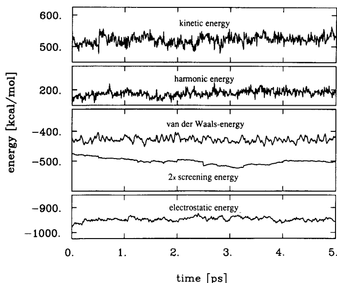
Figure 5 Time dependence of various contributions to the total energy of BPTI resulting from molecular dynamics simulation B as described in Section 3.2. The screening contribution is scaled by a factor of 2. In the simulation the screening potential \delta\Phi(\mathbf{R}_{jk}) was updated and atomic velocities were rescaled (corresponding to T = 300 K) every 250 fs. Because of the coarse updating scheme the screening energy, defined as E_{\text{screening}} = 1/2 \sum_i \delta\Phi(\mathbf{r}_i(t)) (see Equation (25)) exhibits discontinuities. (Parameters for simulation B are in Section 3.2, the discretization scheme used for evaluation of \delta\Phi is defined in Section 2.2.4, parameters for the water continuum model are given in Section 2.2.7; see also Appendix B.)
